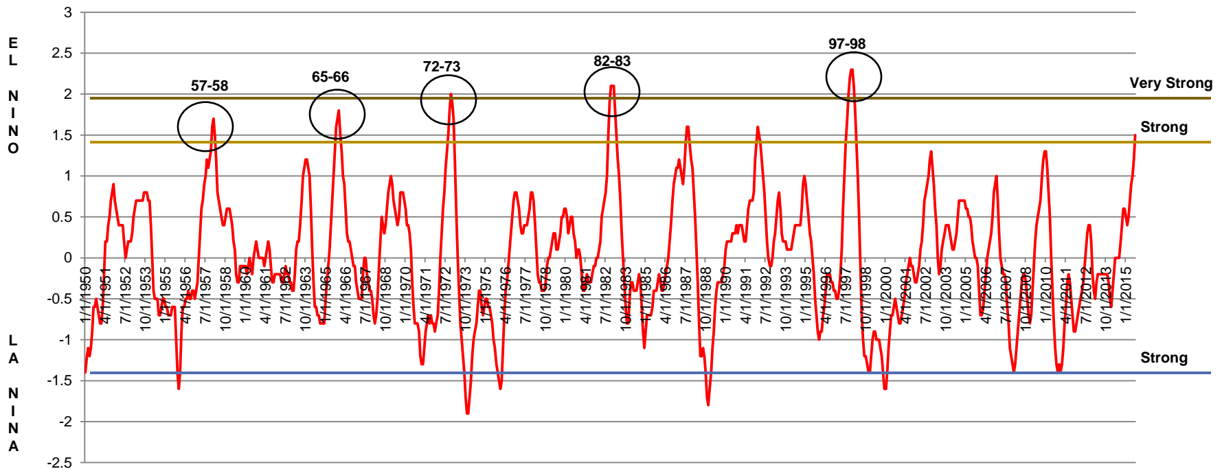
NOAA Climate Prediction Center Oceanic Nino Index ONI
